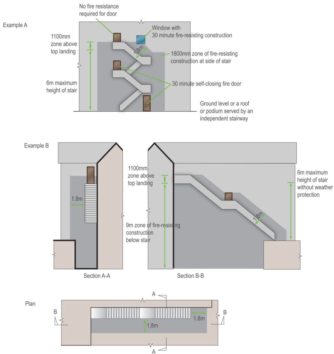
Figure 7: Fire resistance to areas adjacent to external stairs
