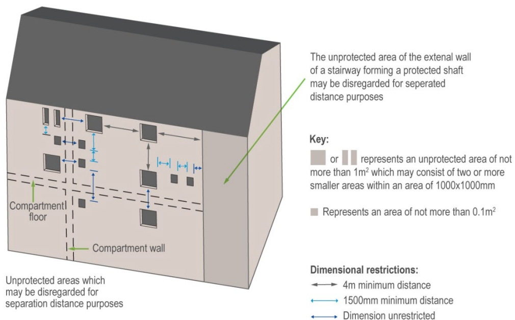
Figure 18: Unprotected areas that may be disregarded in assessing the separation
