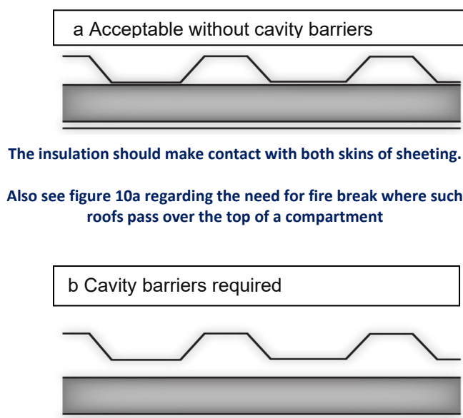
Figure 13: Provisions for cavity barriers in double-skinned insulated roof sheeting
